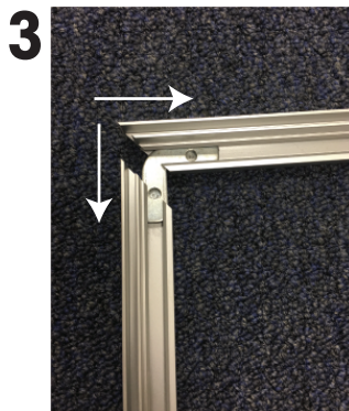
3 Insert joiner pieces into innermost channel of the metal frames.
